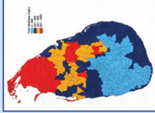
Ground Water Hardness
