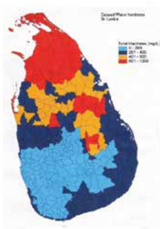
Fig. 2: Distribution of hard water in Sri Lanka Courtesy: Water Resources Board, Sri Lanka
