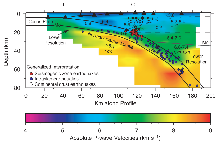
Figure 10. Generalized interpretation of the Nicoya Peninsula 3-D velocity models and associated hypocenters. Colour and values indicate V_P ; V_P/V_S shown in italics. The observed velocities agree well with P -wave velocities and crustal structure (dashed black lines) from wide-angle refraction data (Sallarés et al. 2001). The updip limit of interplate seismicity (red circles) may correspond to the mid crust/oceanic slab interface, identified by the transition from 5.8 to 6.4 \text{km s}^{-1} P -wave velocities. The continental Moho (Mc) appears between 32 and 40 km depth BSL, and the downdip limit of microseismicity clearly occurs updip of the continental Moho/oceanic slab intersection. The forearc mantle wedge may be 15–30 per cent hydrated based on decreased P -wave velocities and slightly elevated V_P/V_S . The oceanic Moho (Mo) is well resolved, and oceanic mantle P -wave velocities are normal with slightly elevated V_P/V_S .
