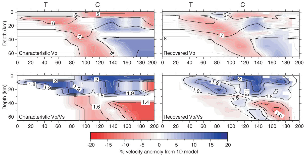
Figure 6. Representative cross-section along Profile 4 (shown in Fig. 3) through the characteristic V_P and V_P/V_S velocity models (column 1), and the recovered V_P and V_P/V_S models (column 2). Colours represent velocity anomaly from the initial 1-D velocity model; contours represent absolute V_P or V_P/V_S . T and C represent the MAT and coastline locations, respectively. Features discussed in text marked with dashed lines.
